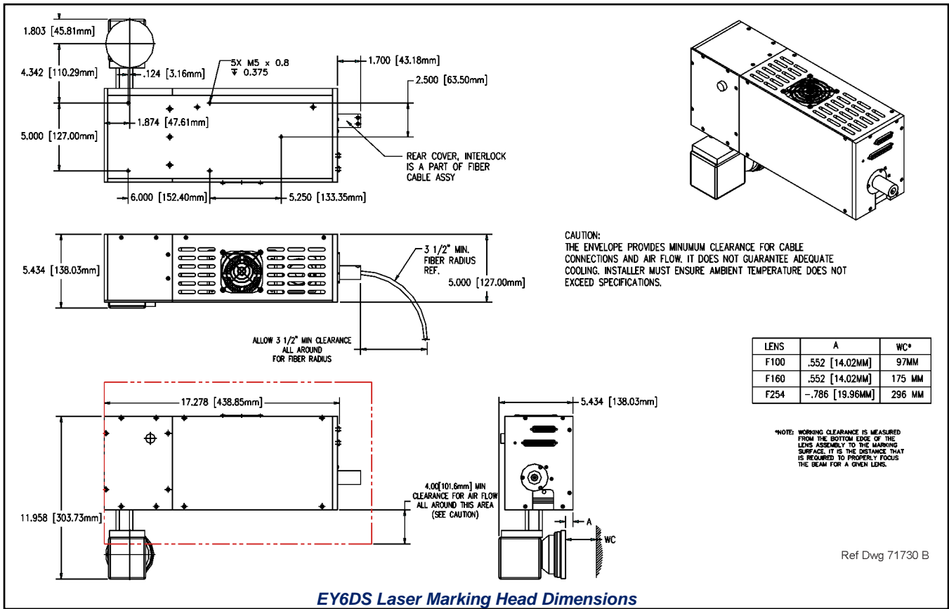
EY6DS Laser Marking Head Dimensions
