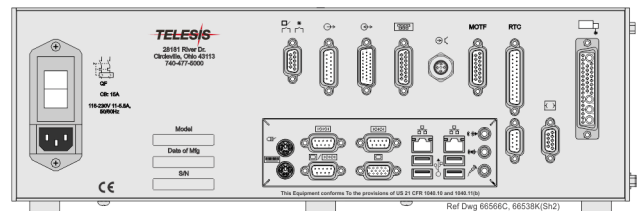
C1060 Laser Controller Back Panel – Embedded Computer
