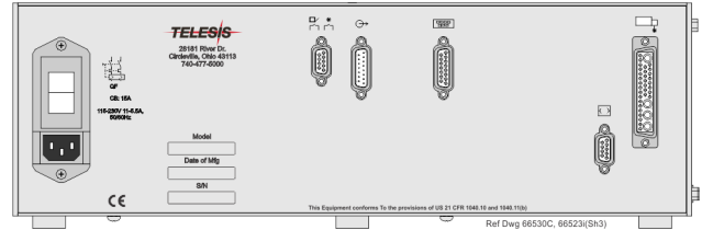
C1060 Laser Controller Back Panel – External Computer
